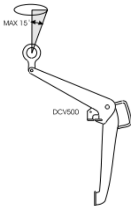
Figure 1 - The maximum chain sling angle must not exceed 15°
