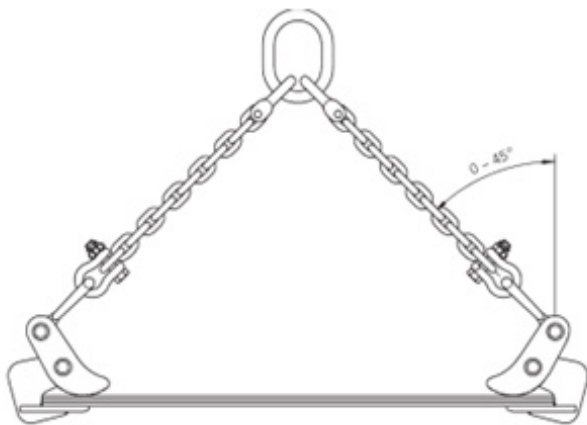
Figure 1 - Maximum chain sling angle
